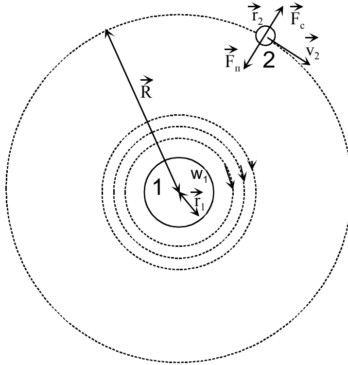
Figure : Two-dimensional model of gravitational interaction of two bodies. Forces operating on a body 2 are specified. The F_c -centrifugal force, F_p -force of an attraction of a body 2 from a body 1, v_2 – the linear speed of a body 2 on an orbit, R – the radius of an orbit, r_1 – the radius of a body 1, r_2 – the radius of a body 2, w_1 – the angular speed of rotation of air on a surface of a body 1, m_2 – body weight 2.
